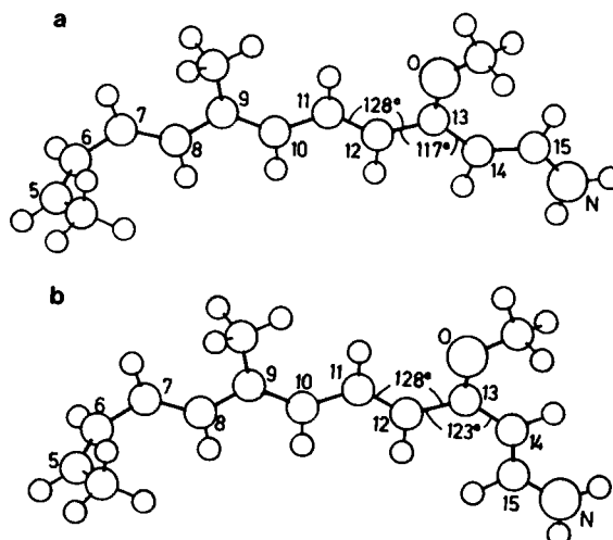
FIGURE 4 MNDOC geometry of 13-OCH 3 -RET-NH 3 + is shown; (a) all- trans , (b) 13- cis .
