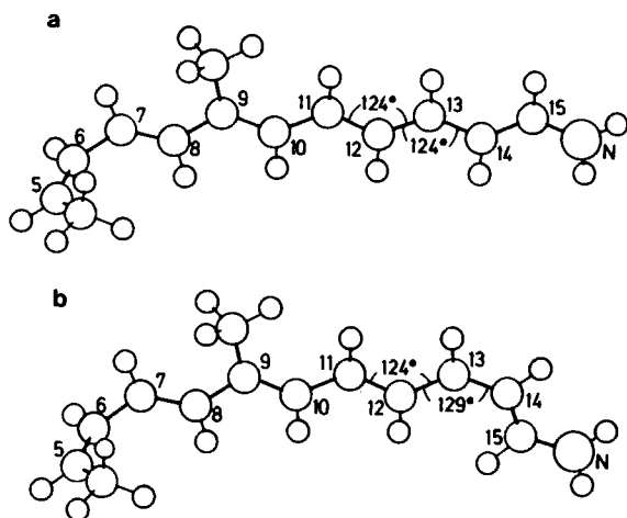
FIGURE 3 The equilibrium geometry of the protonated Schiff-base 13-H-RET-NH 3 + is drawn to scale as obtained from the MNDOC method; (a) all- trans , (b) 13- cis .
