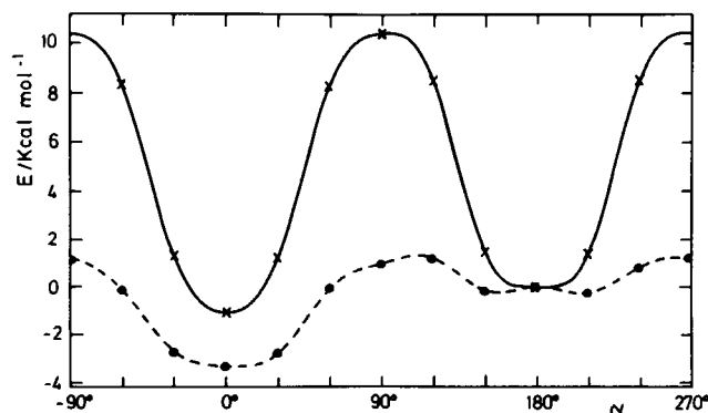
FIGURE 5 The effect of 13-methoxy substitution on R_{13} isomerization potential curves for the model retinal Schiff-bases 13-X-RET-NH 2 + is shown; X = CH 3 (—); X = OCH 3 (---); the curves represent a cubic spline interpolation of the numerical values calculated at 30° intervals; all- trans is at a torsion angle \alpha of 180°, 13- cis is at 0°.
