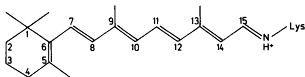
FIGURE 1 The Schiff base of retinal is shown. The chromophore is attached through the terminal nitrogen to a lysine residue of BR.
